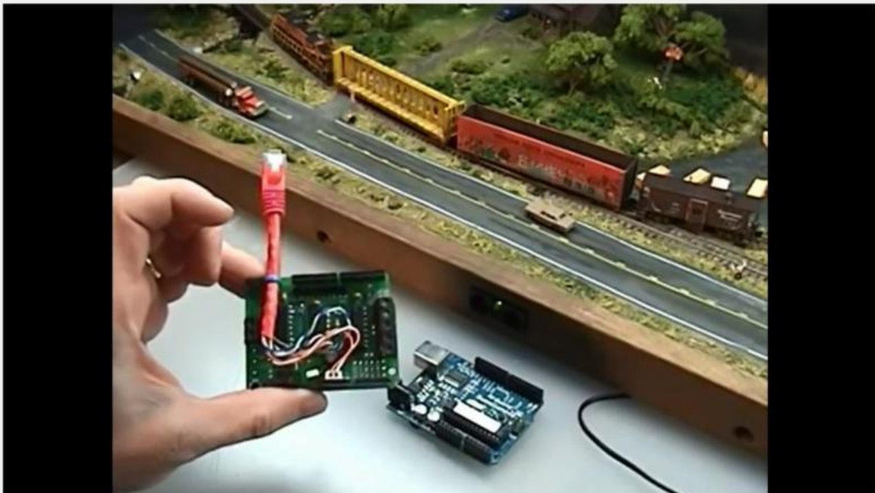
Arduino Control of Model Train
